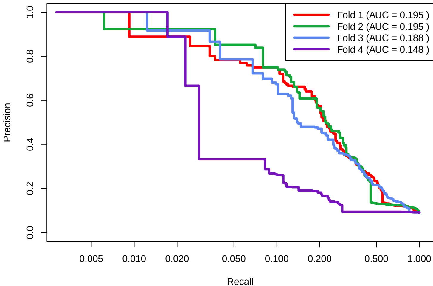
SPELL Original Datasets: 0.0 Validation
