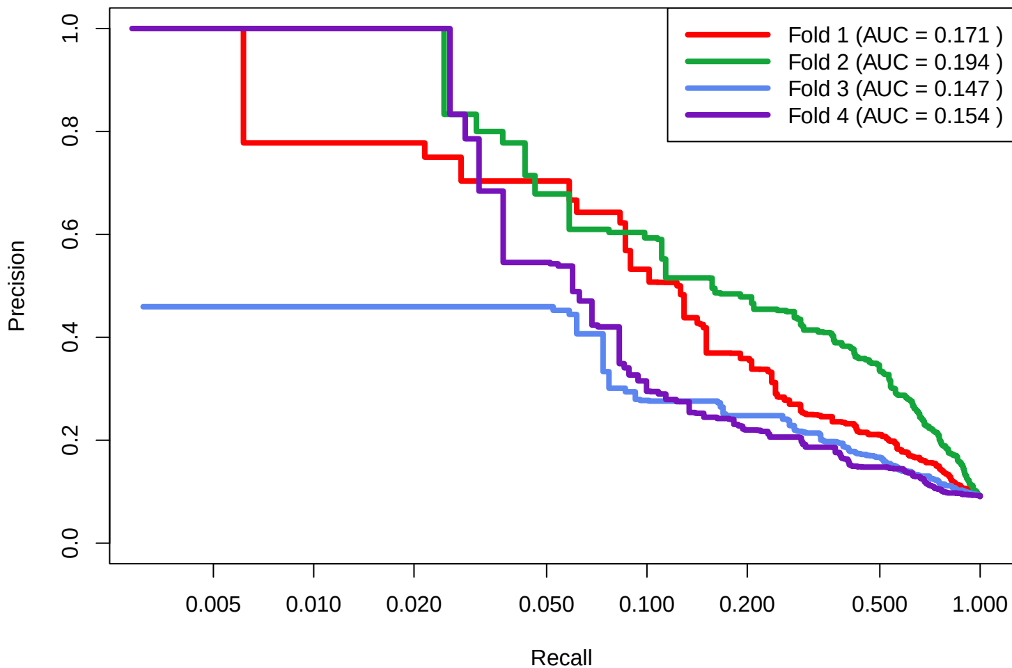
SPELL Original Datasets: 0.50 Validation
