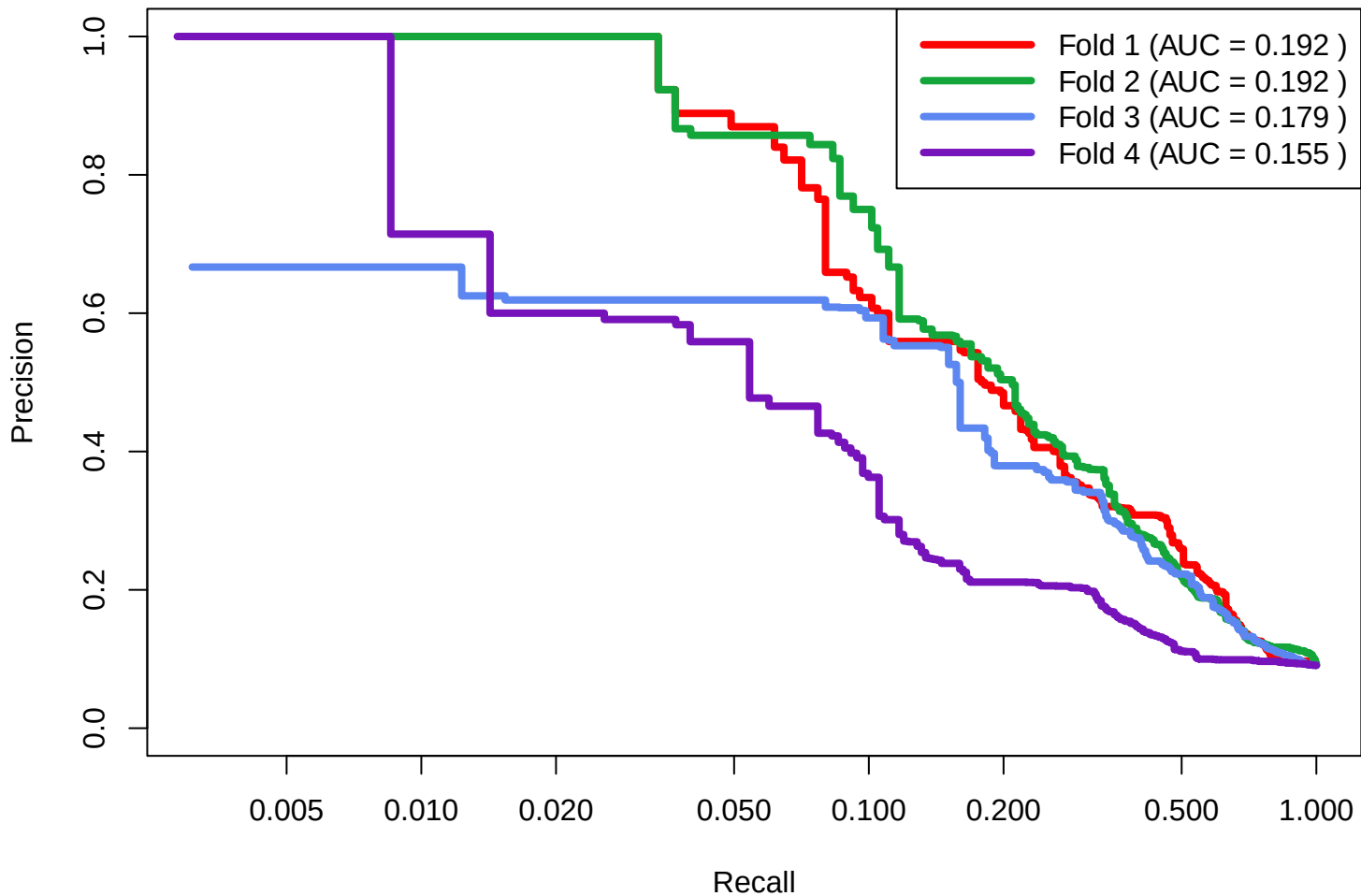
SPELL Original Datasets: 0.20 Validation
