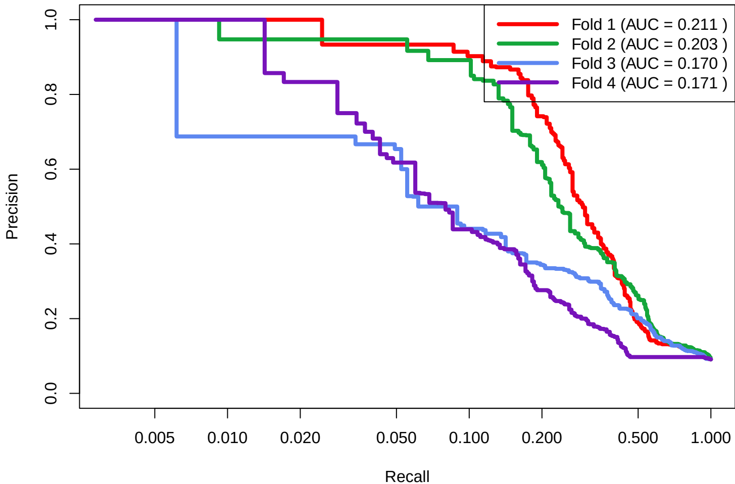
SPELL Original Datasets: 0.05 Validation
